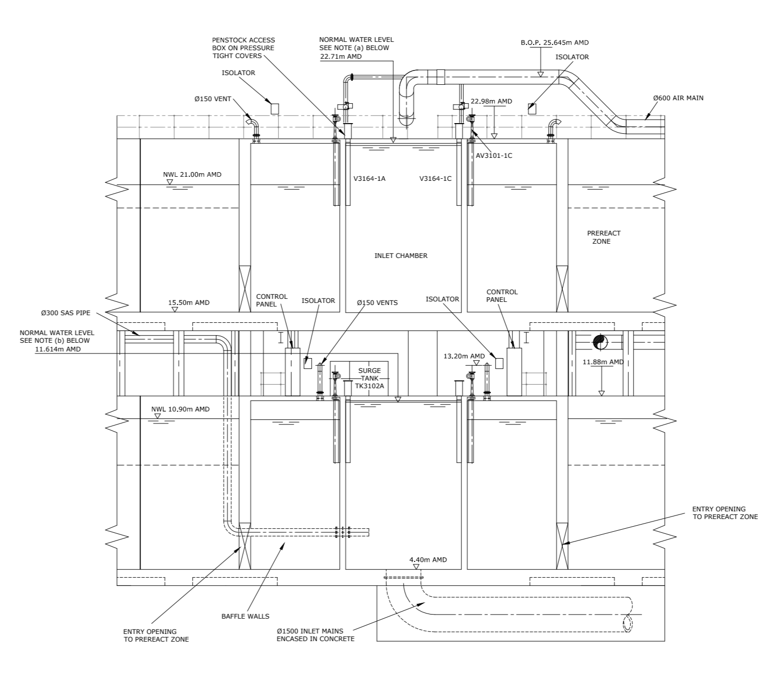
SECTION C-C
